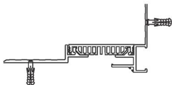
AR215-080 KÖŞE DETAYI AR215-080 CORNER DETAIL
